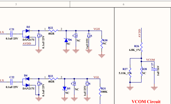
VCOM Circuit
