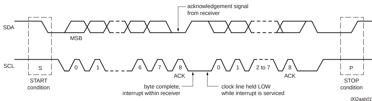
Fig 18. Data transfer on the I 2 C-bus
