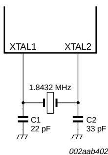
Fig 15. Crystal oscillator circuit reference
