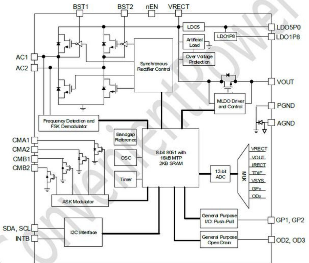
Figure 9: CPS3008 Function Block Diagram
